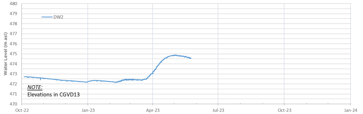
Figure B.47: Hydrograph of water levels at Domestic Well DW2, masl.
