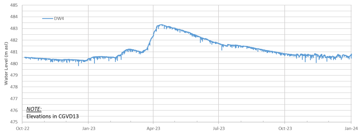
Figure B.49: Hydrograph of water levels at Domestic Well DW4, masl.
