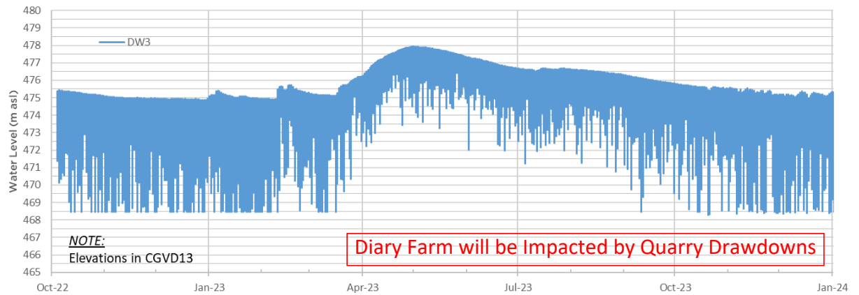
Figure B.48: Hydrograph of water levels at Domestic Well DW3, masl.
